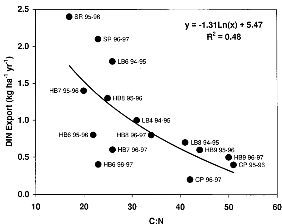
Figure 4. Regression of streamwater DIN exports (kg ha -1 yr -1 ) on streamwater C:N ratio. Points represent the mean annual value for each site.
